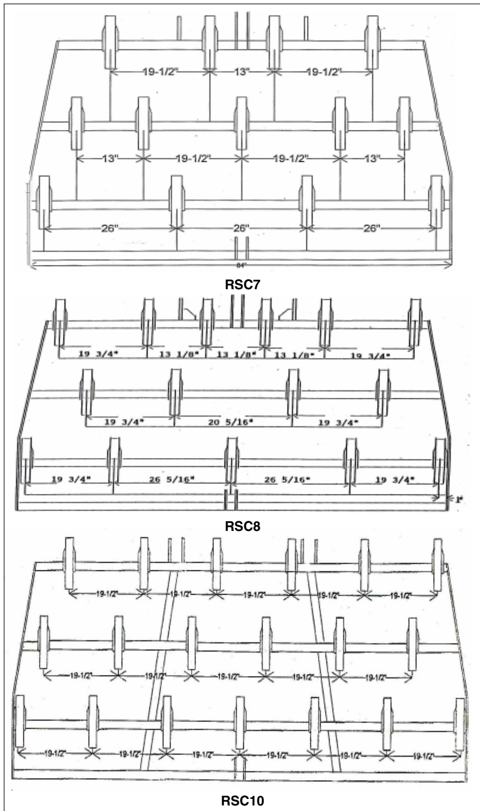
Fig. 14 TINE LOCATIONS
