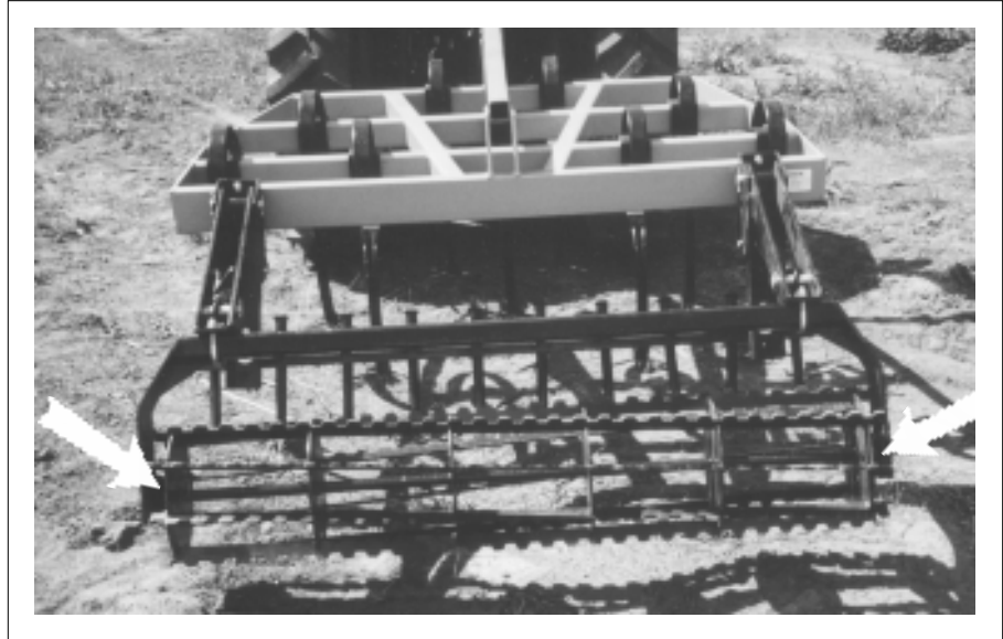
Fig. 9 CRUMBLER ROLLER BEARINGS
