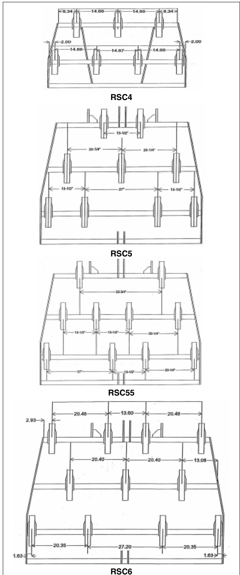
Fig. 13 TINE LOCATIONS
