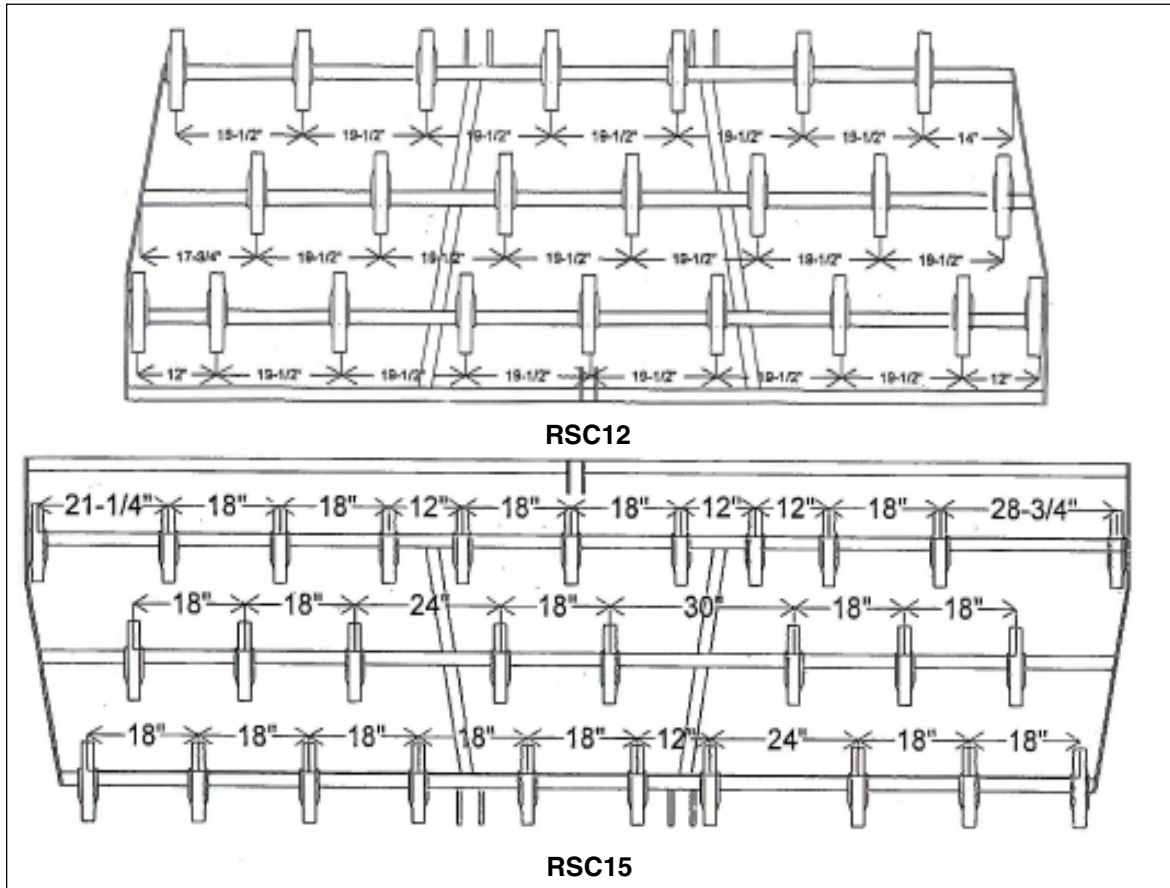
Fig. 15 TINE LOCATIONS
