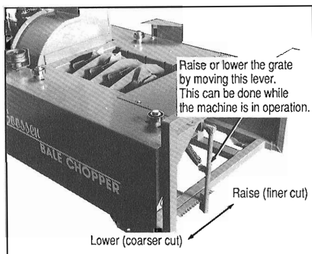
Figure 13. Depth-of-Cut Adjustment (Blower Models)
