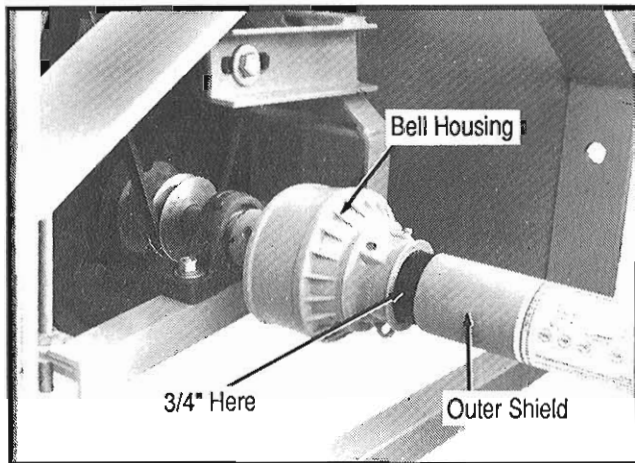
Figure 4. PTO Drive Shaft Installation
