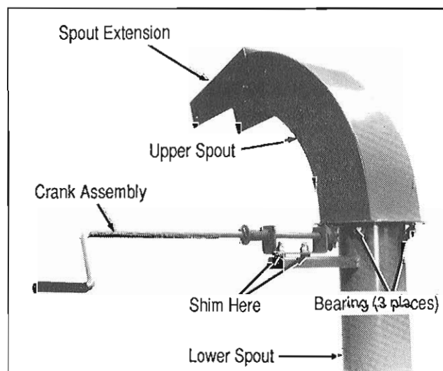
Figure 3. Spout Attachment & Crank Assembly
