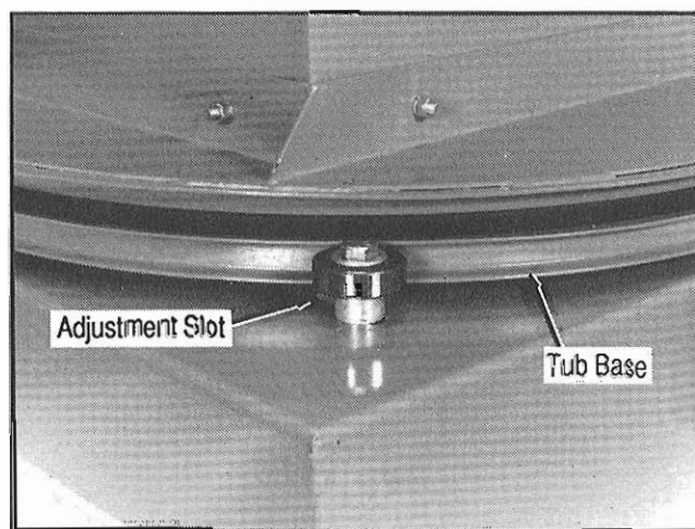
Figure 14. Tub Carrier Bearing Position
